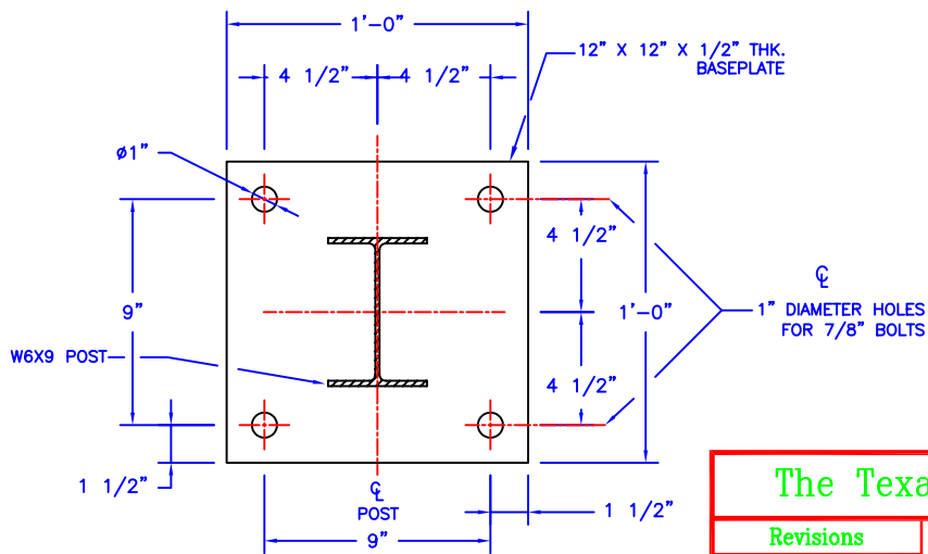
W6x9 BASEPLATE DETAILS
