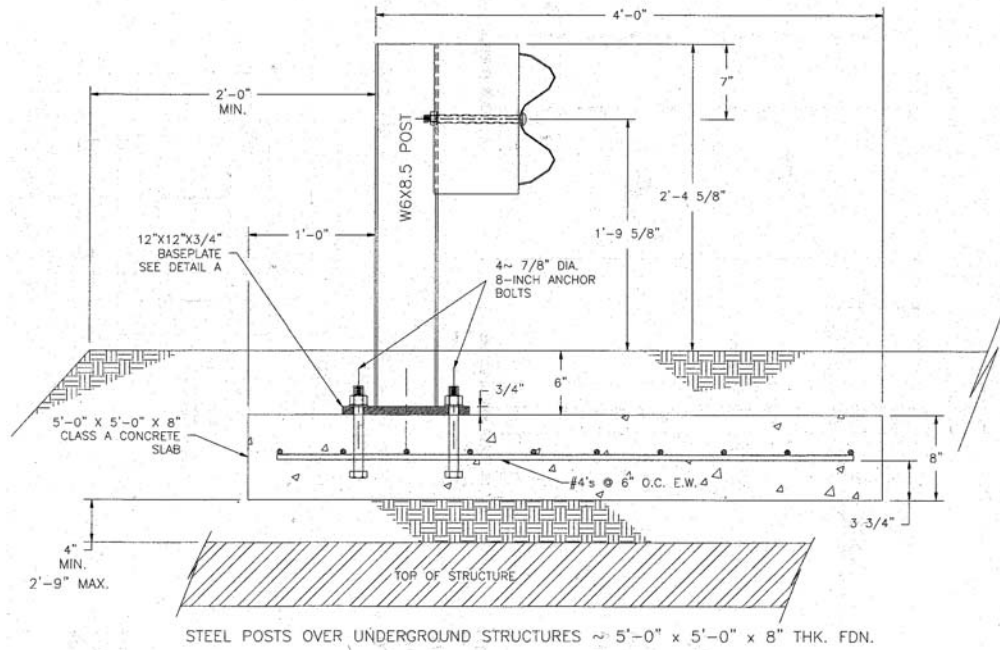
Figure 2. 5 ft x 5 ft Footing Cross-Section.
