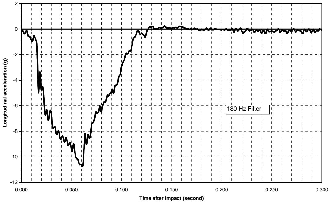
Figure E3. Accelerometer trace for test 405160-12 P2.
