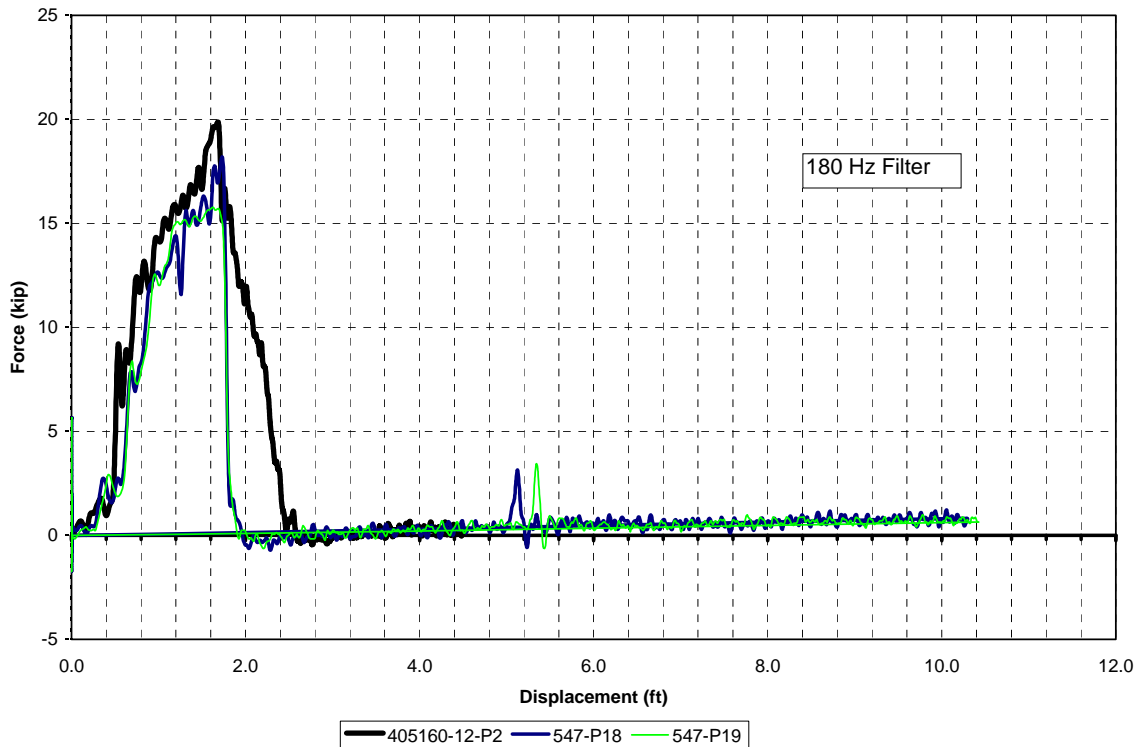
Figure 5. Force versus displacement comparison for post on 4 ft x4 ft slab and posts in strong soil.
