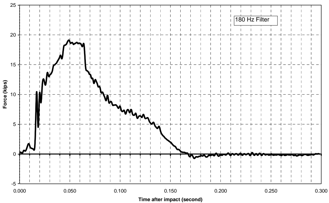
Figure E2. Force trace for test 405160-12 P1.
