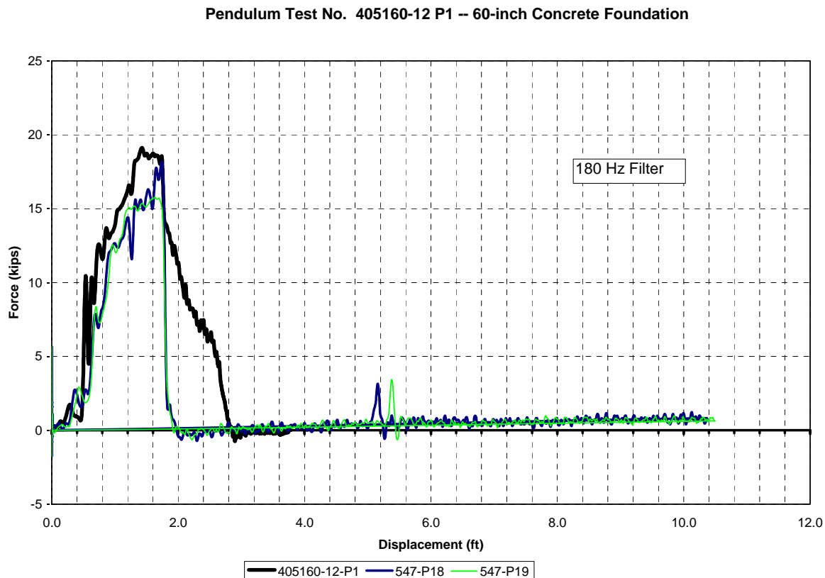
Figure 4. Force versus displacement comparison for post on 5 ft x 5 ft slab and posts in strong soil.
