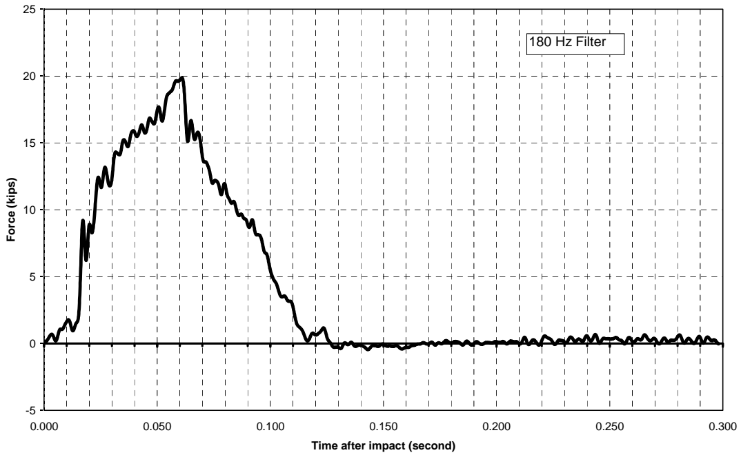
Figure E4. Force trace for test 405160-12 P2.
