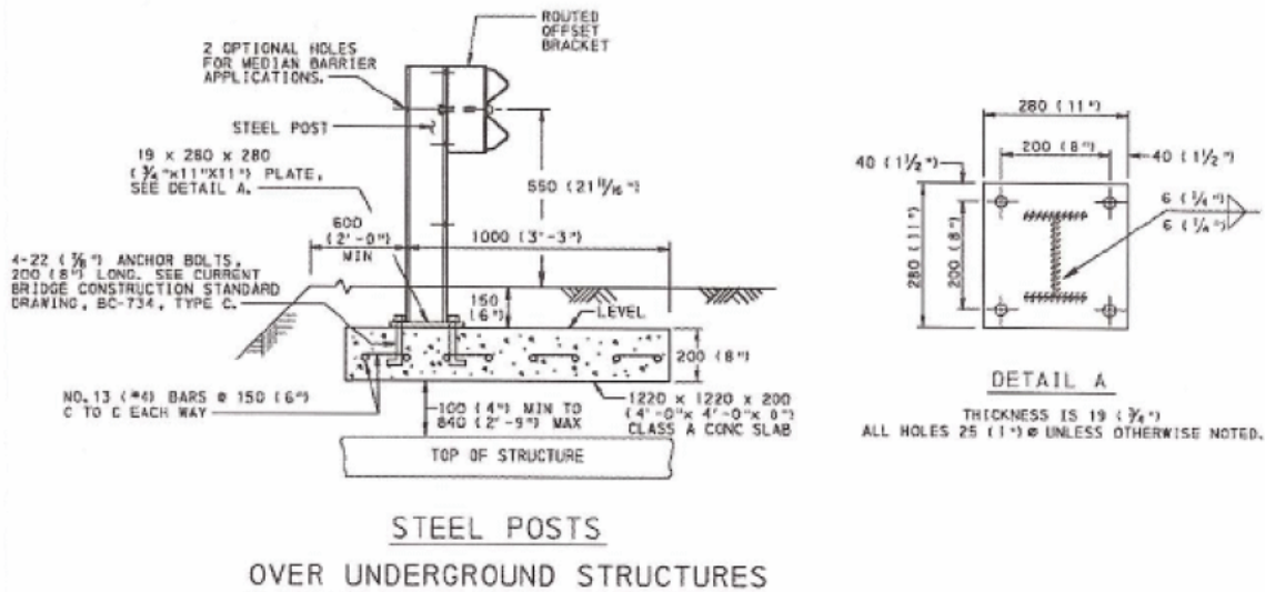
Figure 1. Steel Post Over Underground Structures.
