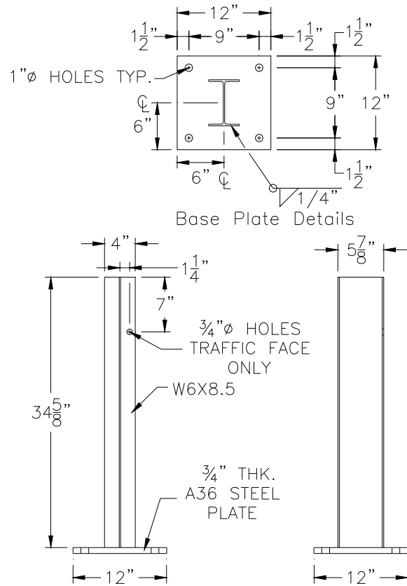
Figure 3. Steel Post Details.
