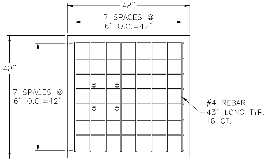
TOP VIEW BOLT DETAIL B
