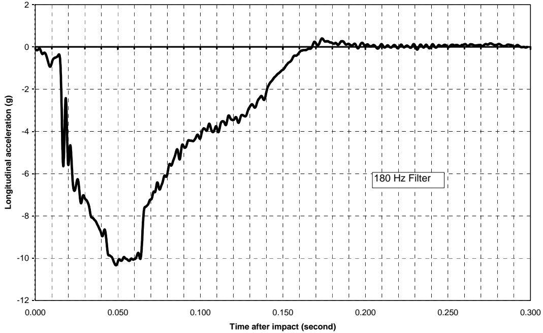
Figure E1. Accelerometer trace for test 405160-12 P1.
