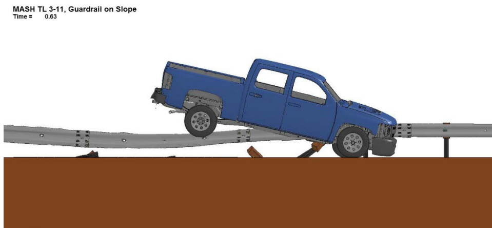
Figure 1.31. Case 2 Silverado model at maximum pitch.
