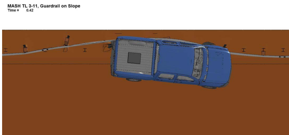
Figure 1.32. Case 2 Silverado model at maximum yaw.
