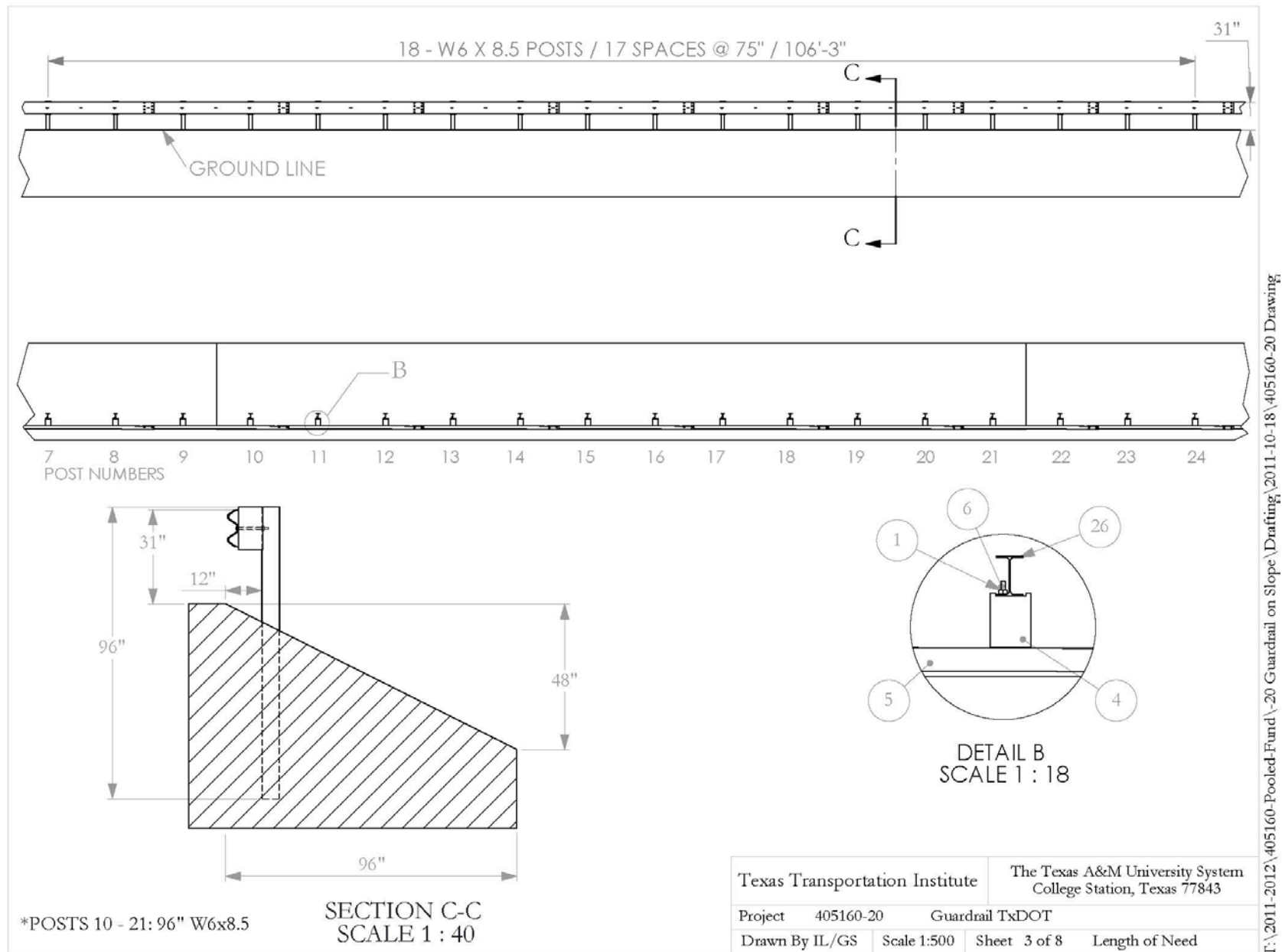
Figure 2.1. Layout of the guardrail on slope.
