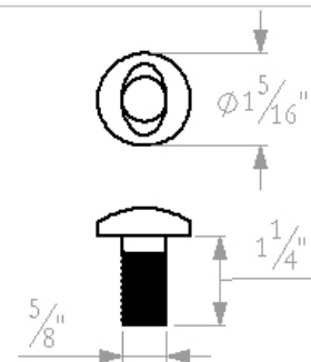
2. Button-head Splice Bolt ARTBA # FBB03
