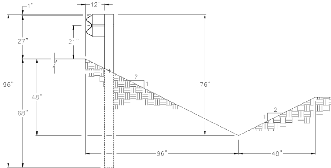
SECTION A-A W6X8.5 STEEL POSTS, 8' LONG W/ 6"x8"x14" ROUTED WOOD BLOCKOUTS
