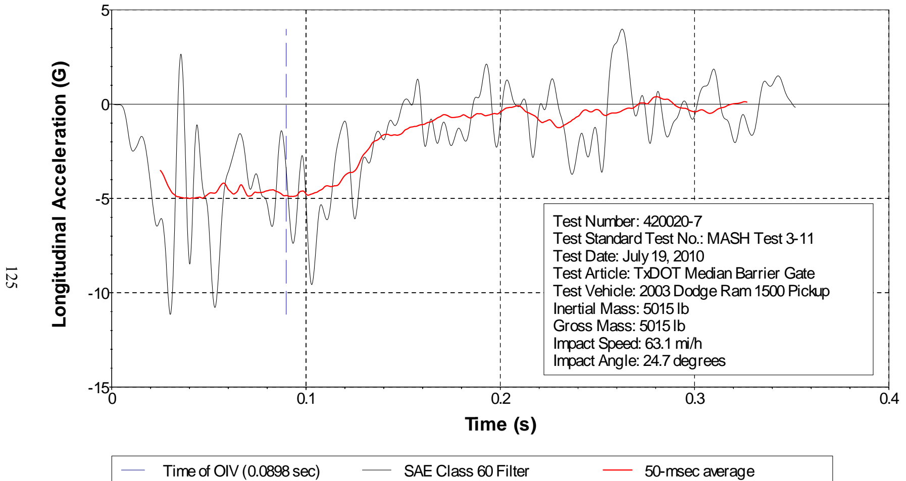
Figure E9. Vehicle Longitudinal Accelerometer Trace for Test No. 420020-7 (Accelerometer Located at Center of Gravity).
