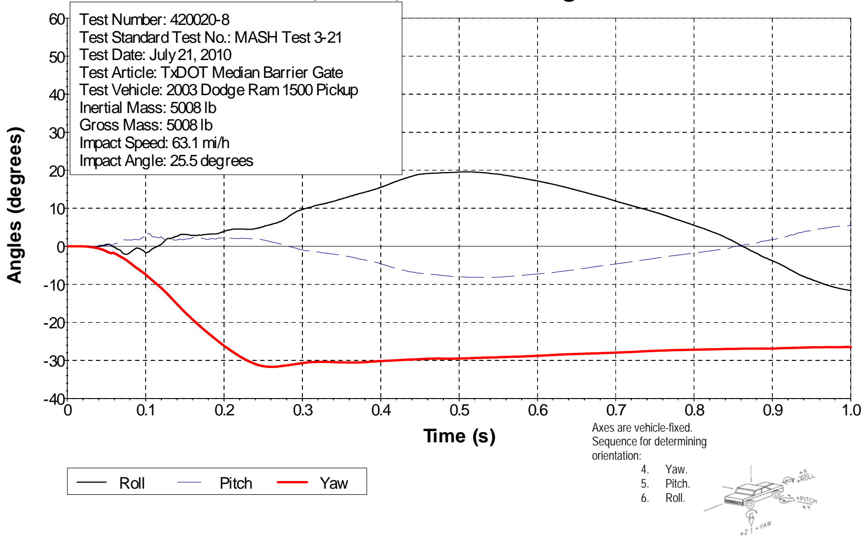
Figure E15. Vehicle Angular Displacements for Test No. 420020-8.
