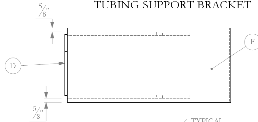
ELEVATION VIEWS
