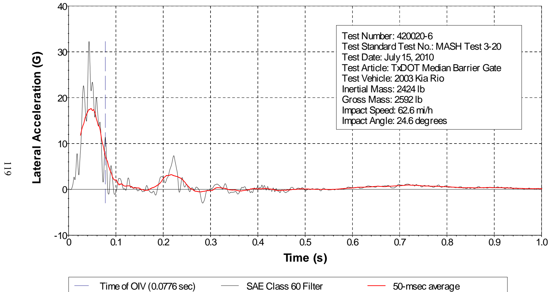
Figure E3. Vehicle Lateral Accelerometer Trace for Test No. 420020-6 (Accelerometer Located at Center of Gravity).
