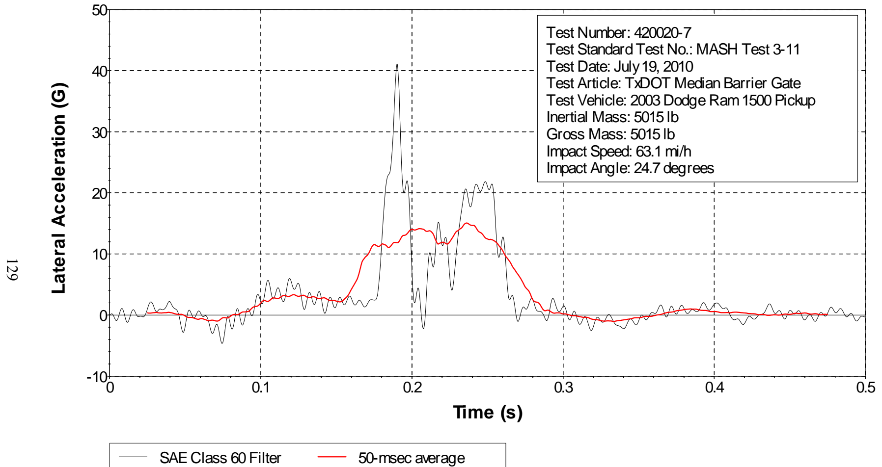
Figure E13. Vehicle Lateral Accelerometer Trace for Test No. 420020-7 (Accelerometer Located over Rear Axle).
