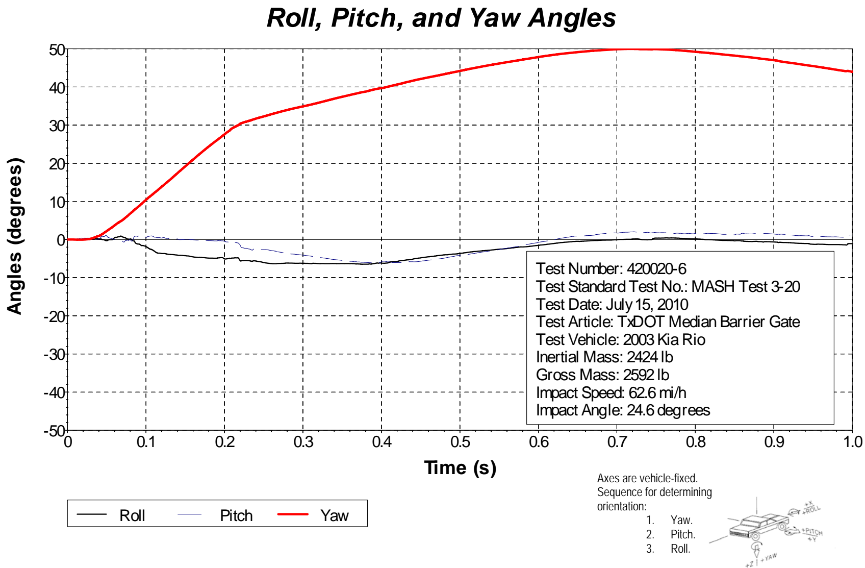
Figure E1. Vehicle Angular Displacements for Test No. 420020-6.
