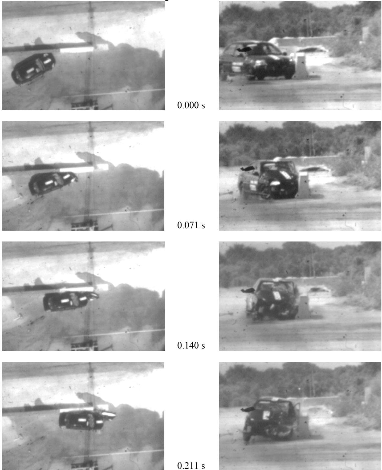
Figure D1. Sequential Photographs for Test No. 420020-6 (Overhead and Frontal Views).
