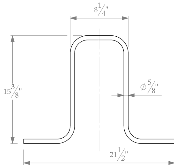
5 STIRRUP FOUNDATION
