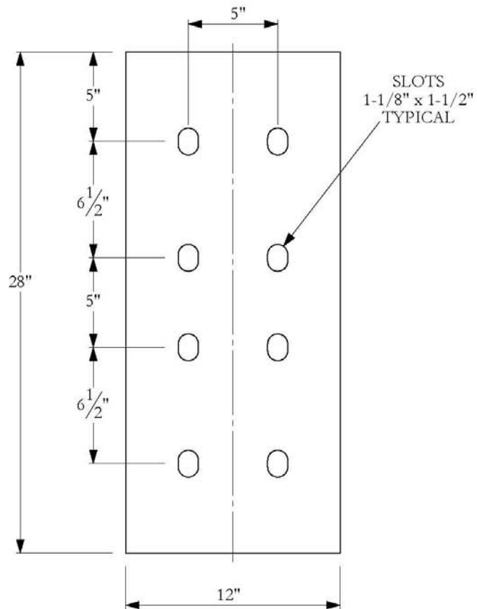
(B) HORIZONTAL PLATE 2 NEEDED PER BRACKET
