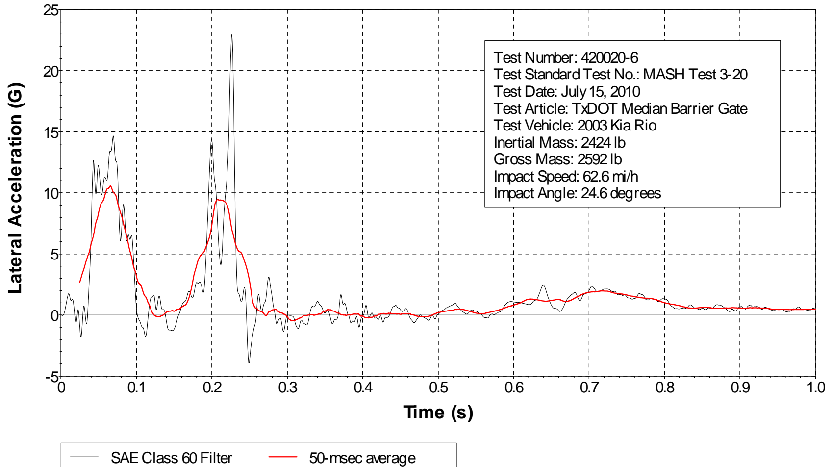
Figure E6. Vehicle Lateral Accelerometer Trace for Test No. 420020-6 (Accelerometer Located over Rear Axle).
