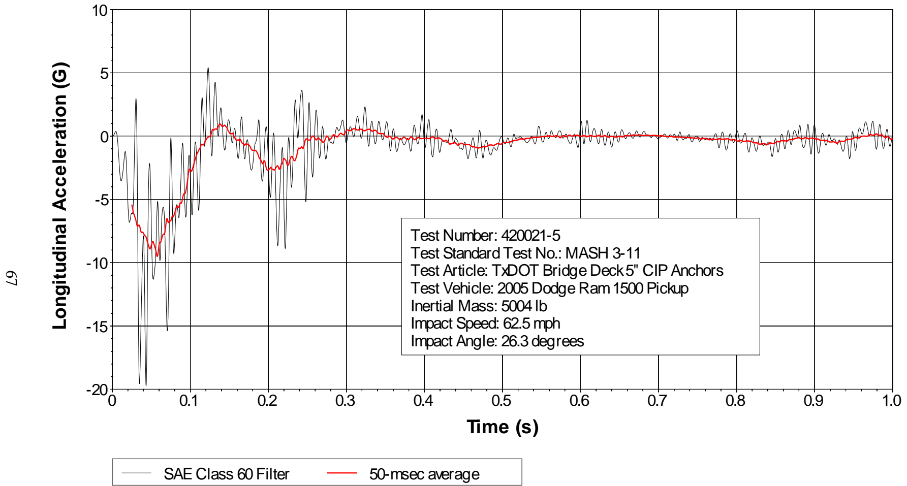
Figure E5. Vehicle Longitudinal Accelerometer Trace for Test No. 420021-5 (Accelerometer Located over Rear Axle).
