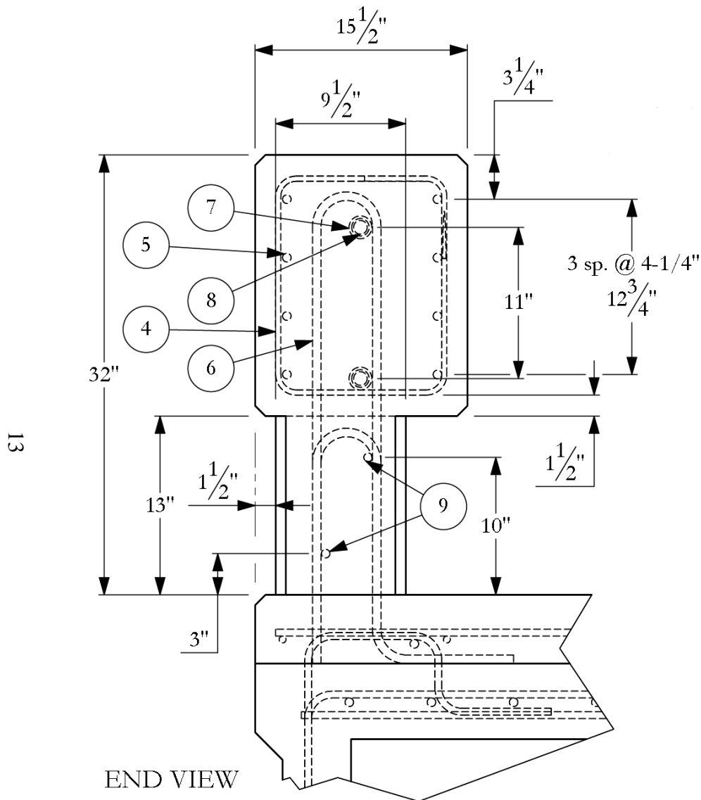
Figure 4.2. Details of the 5-inch CIPD Barrier Anchor Installation.
