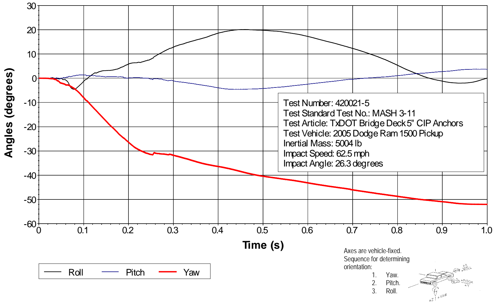
Figure E1. Vehicle Angular Displacements for Test No. 420021-5.
