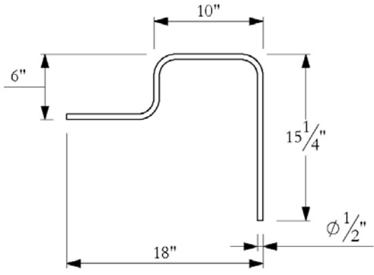
10 Z-BAR SEE NOTE 9a
