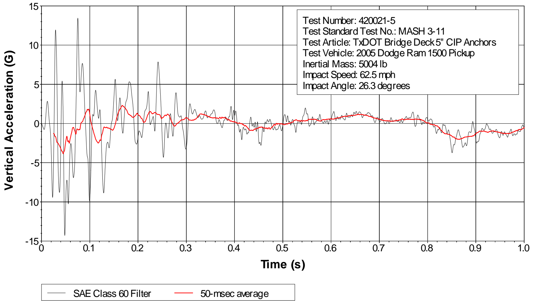
Figure E4. Vehicle Vertical Accelerometer Trace for Test No. 420021-5 (Accelerometer Located at Center of Gravity).
