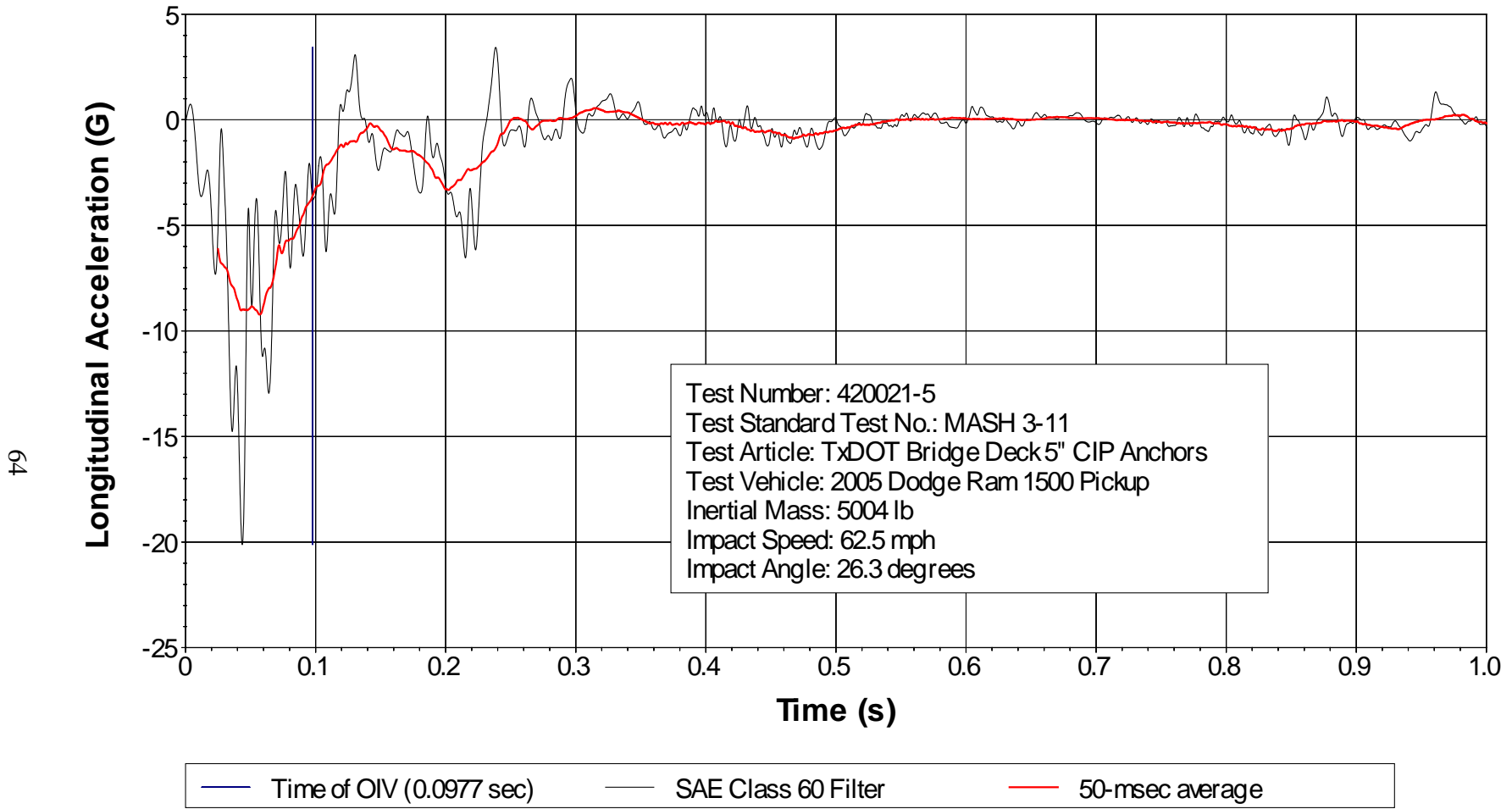
Figure E2. Vehicle Longitudinal Accelerometer Trace for Test No. 420021-5 (Accelerometer Located at Center of Gravity).
