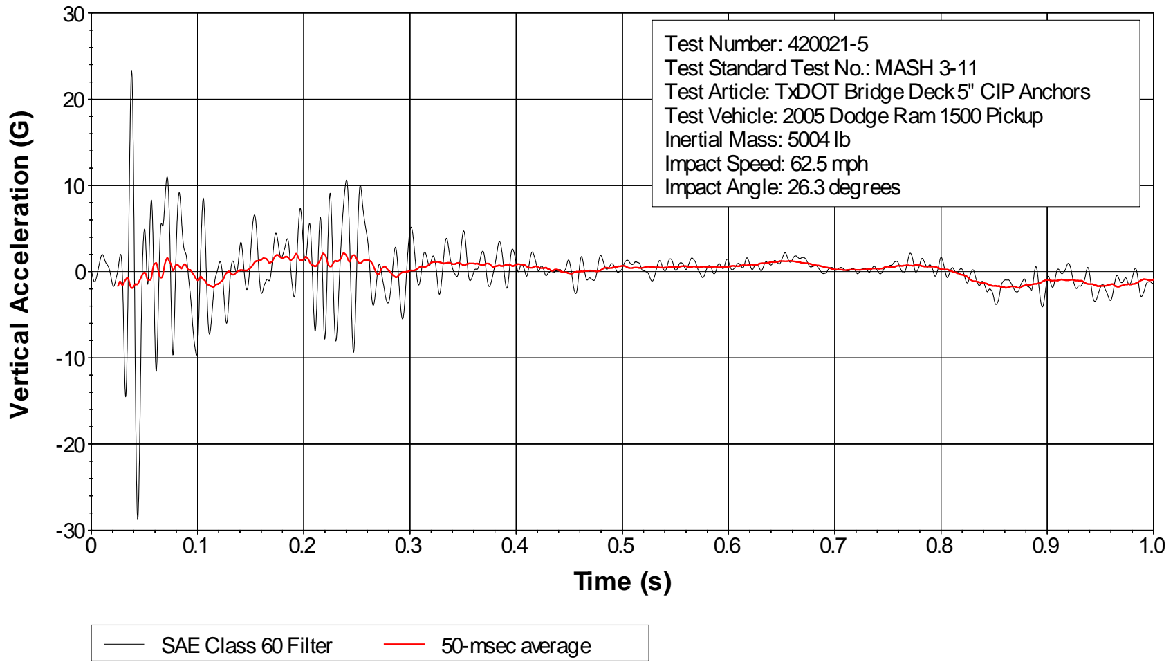
Figure E7. Vehicle Vertical Accelerometer Trace for Test No. 420021-5 (Accelerometer Located over Rear Axle).
