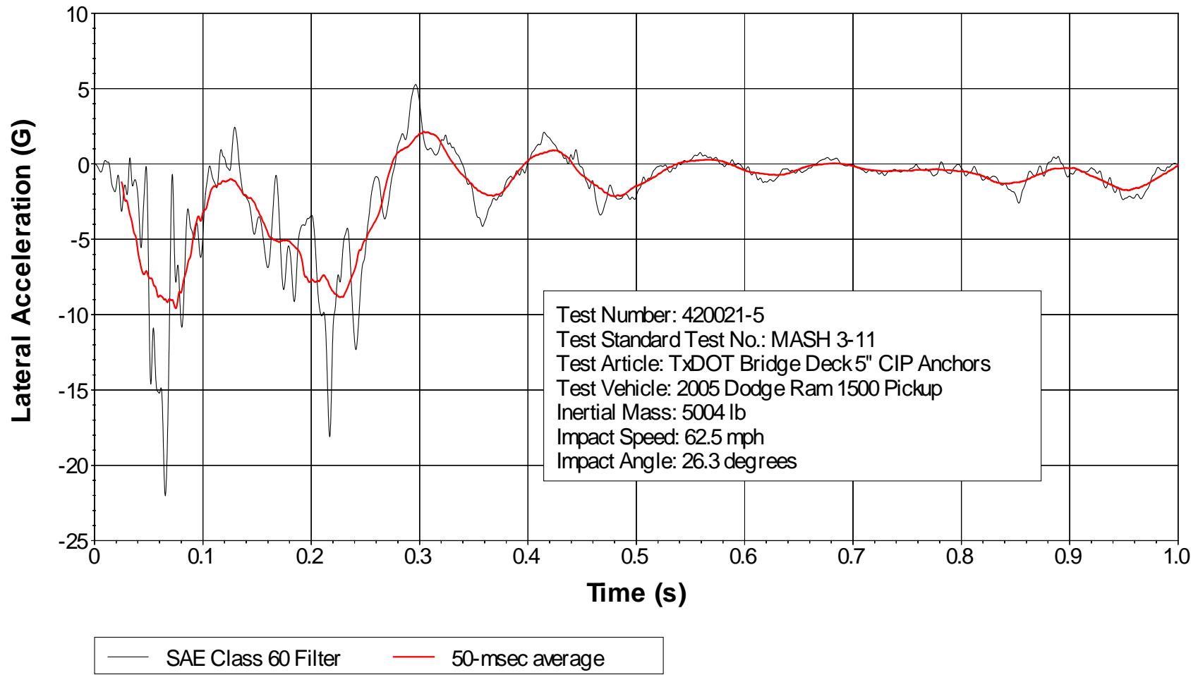
Figure E6. Vehicle Lateral Accelerometer Trace for Test No. 420021-5 (Accelerometer Located over Rear Axle).
