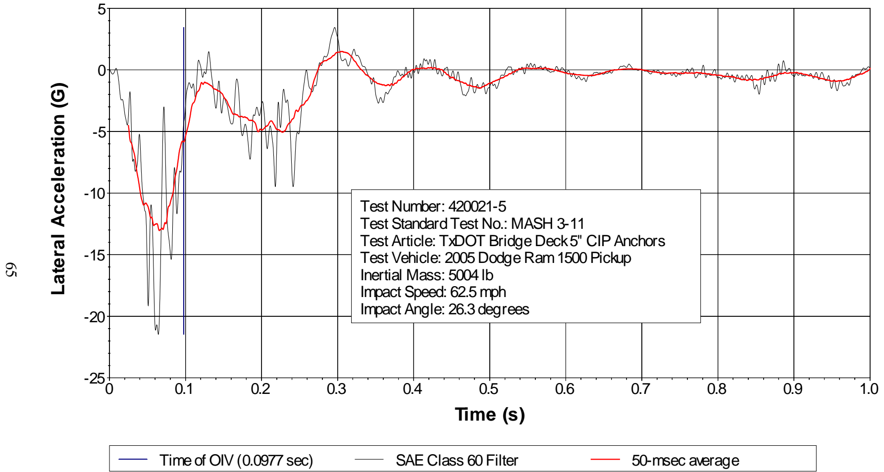
Figure E3. Vehicle Lateral Accelerometer Trace for Test No. 420021-5 (Accelerometer Located at Center of Gravity).
