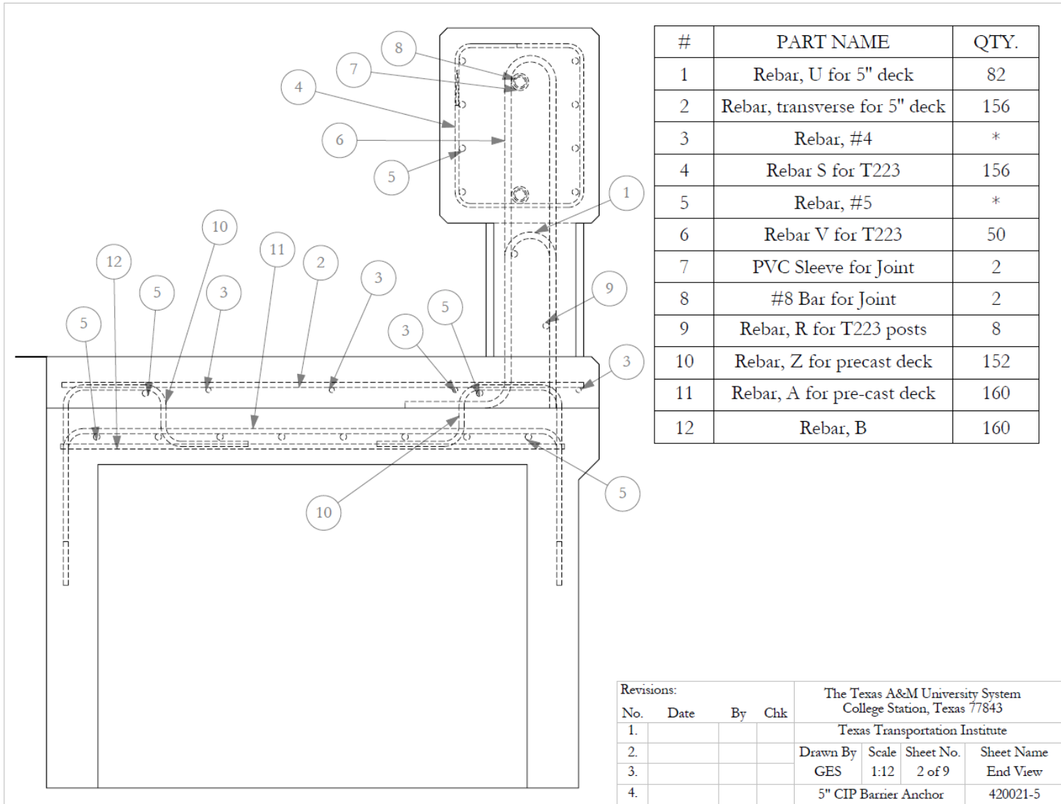
Figure 4.1. Test Article Cross-Section.
