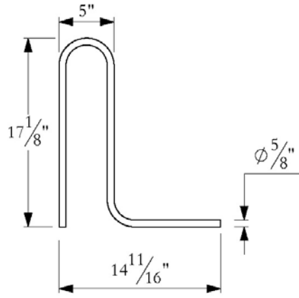
1 U-BAR
