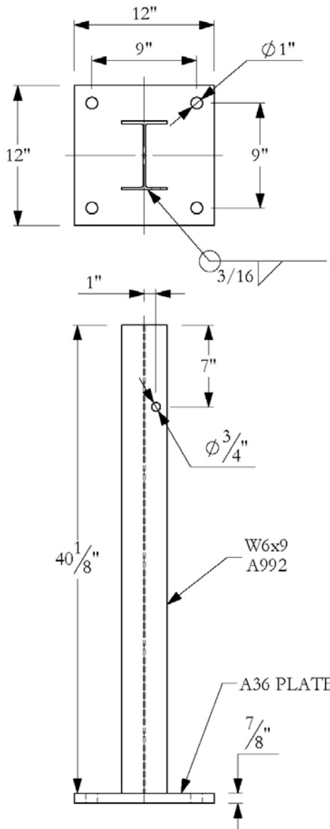
1 BOX CULVERT POST
