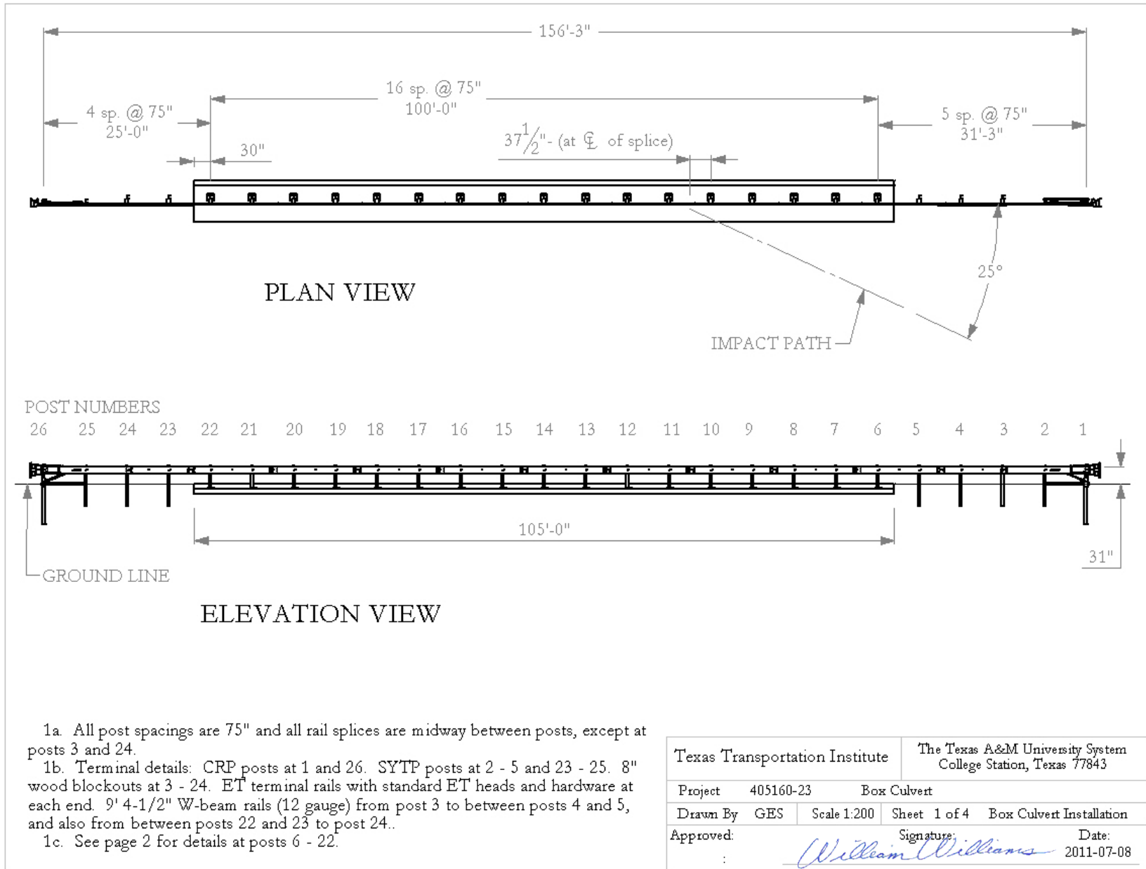
Figure 2.1. Layout of the W-Beam Guardrail on Low-Fill Box Culvert.
