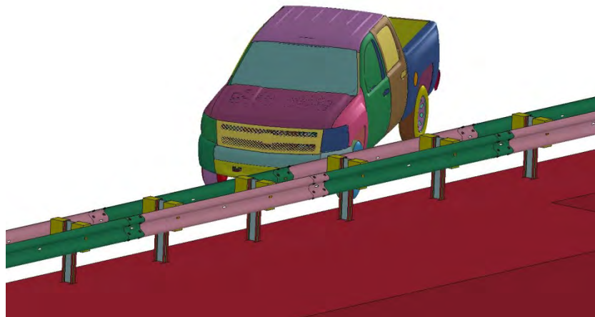
Figure 2.4. Model of the 31-Inch Median W-Beam Guardrail with the 2270P Vehicle Model.
