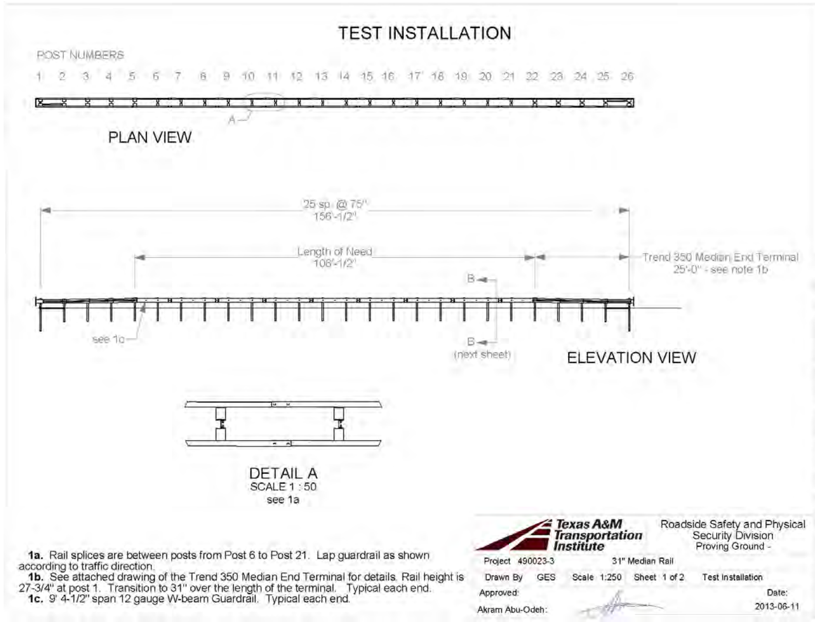
Figure 3.1. Layout of the TxDOT 31-Inch W-Beam Median Barrier.
