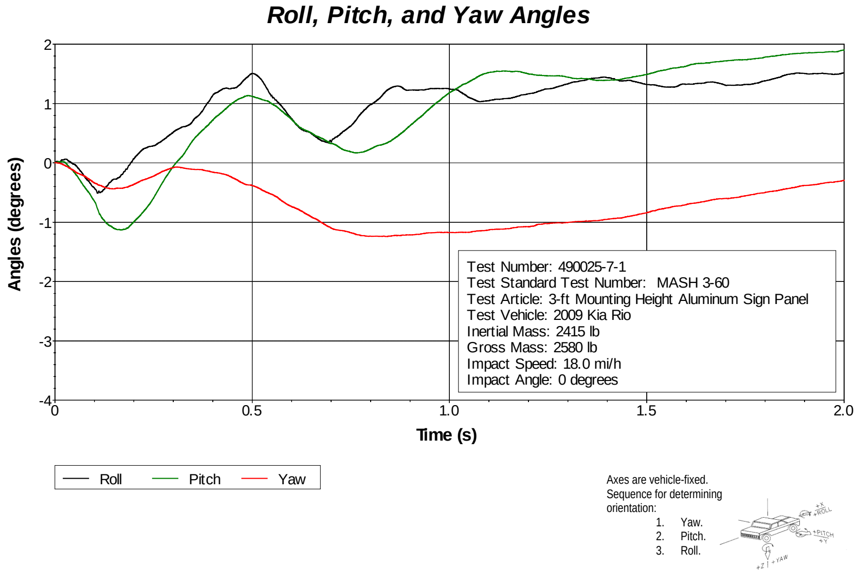
Figure B.2. Vehicle Angular Displacements for Test No. 490025-7-1.
