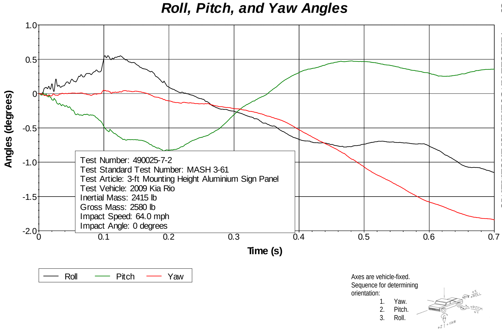
Figure C.2. Vehicle Angular Displacements for Test No. 490025-7-2.
