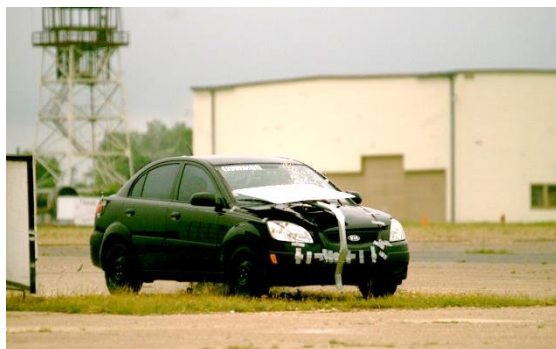
Figure C.1. Sequential Photographs for Test No. 490025-7-2 (Frontal Views).
