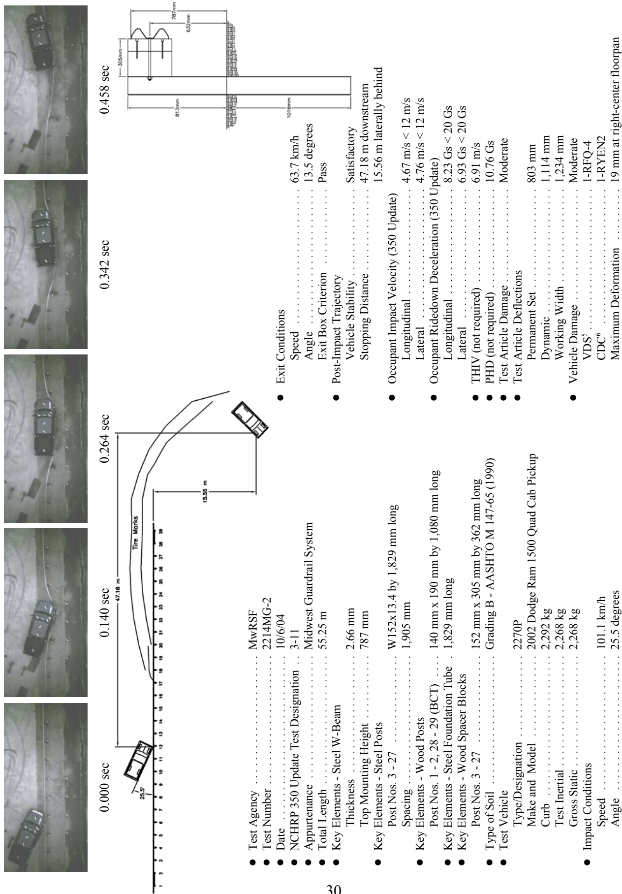
Figure 14. Summary of Test Results and Sequential Photographs, Test 2214MG-2
