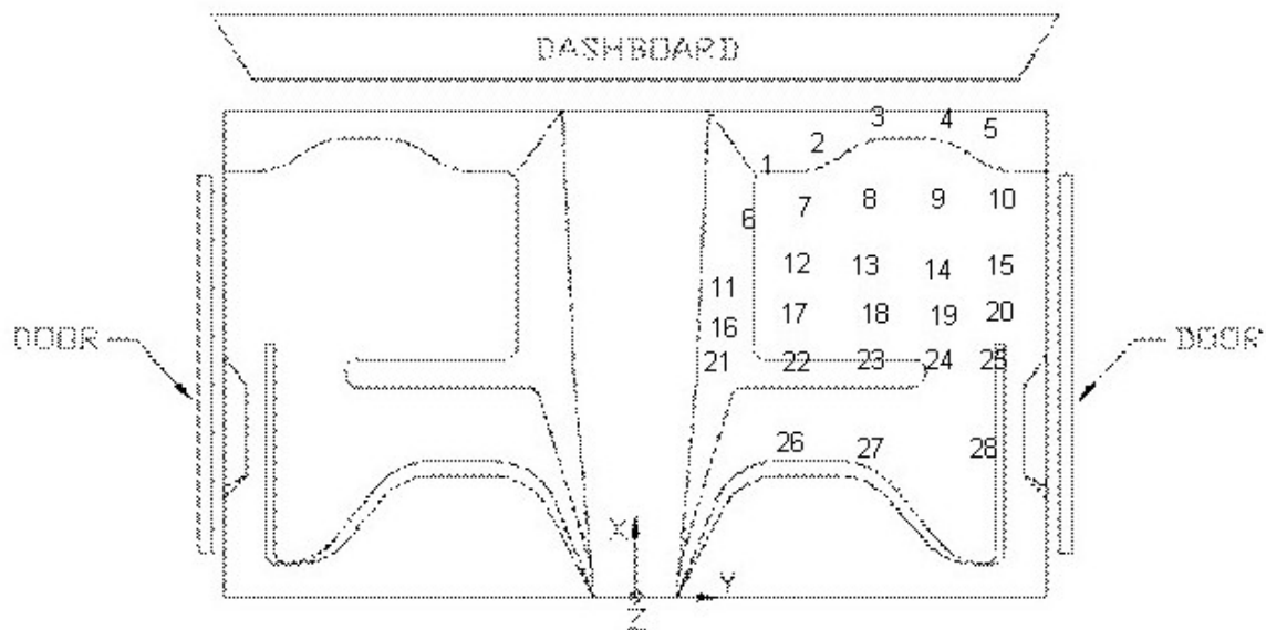
Figure C-1. Occupant Compartment Deformation Data - Set 1, Test 2214MG-2
