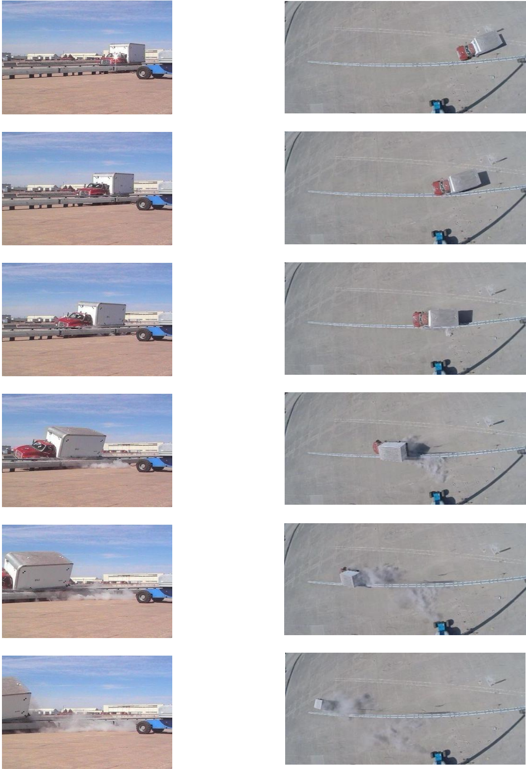
Figure 108. Documentary Photographs, Test No. SFH-3
