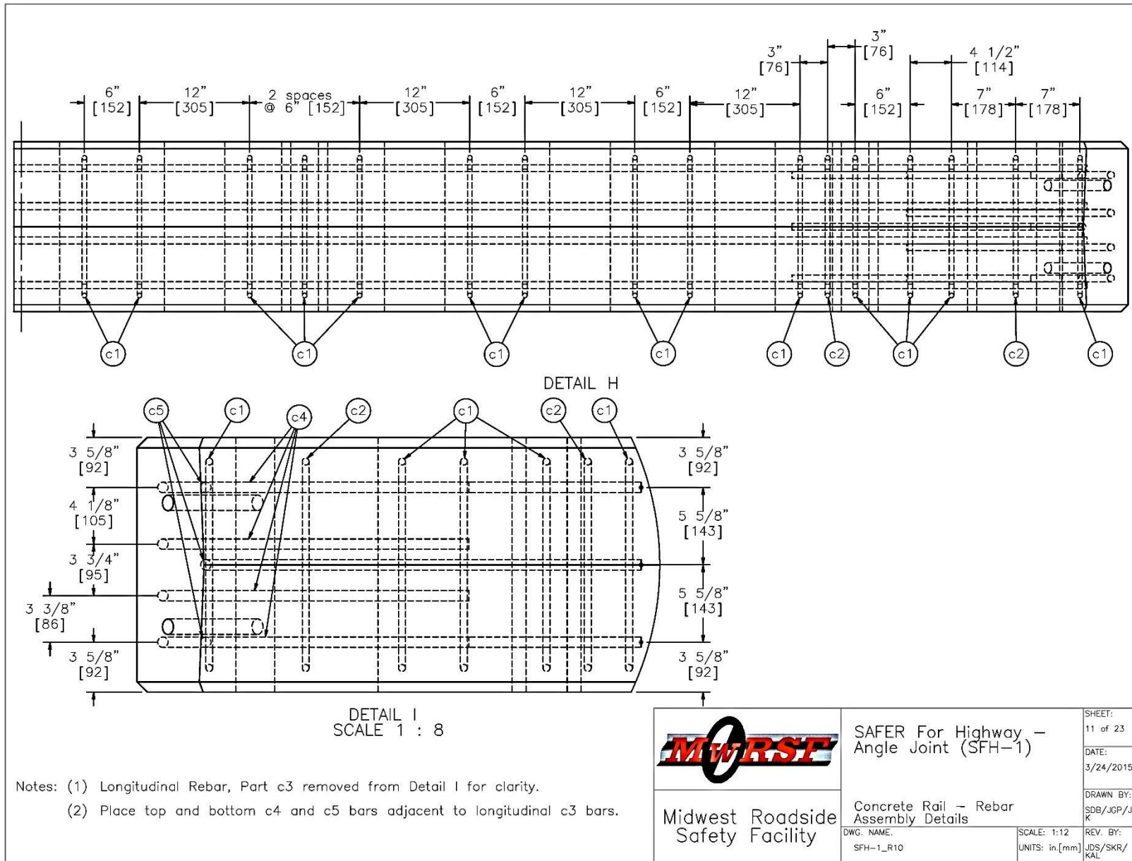
Figure 12. Concrete Beam, Rebar Assembly Details, Test Nos. SFH-1 and SFH-2
