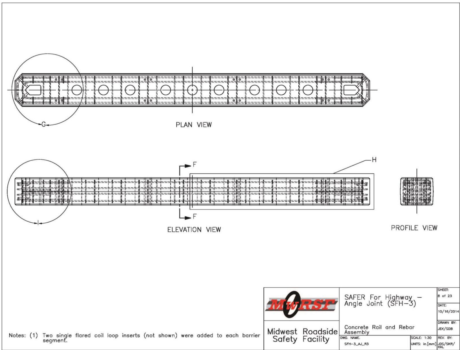
Figure 86. Concrete Beam and Rebar Assembly, Test No. SFH-3
