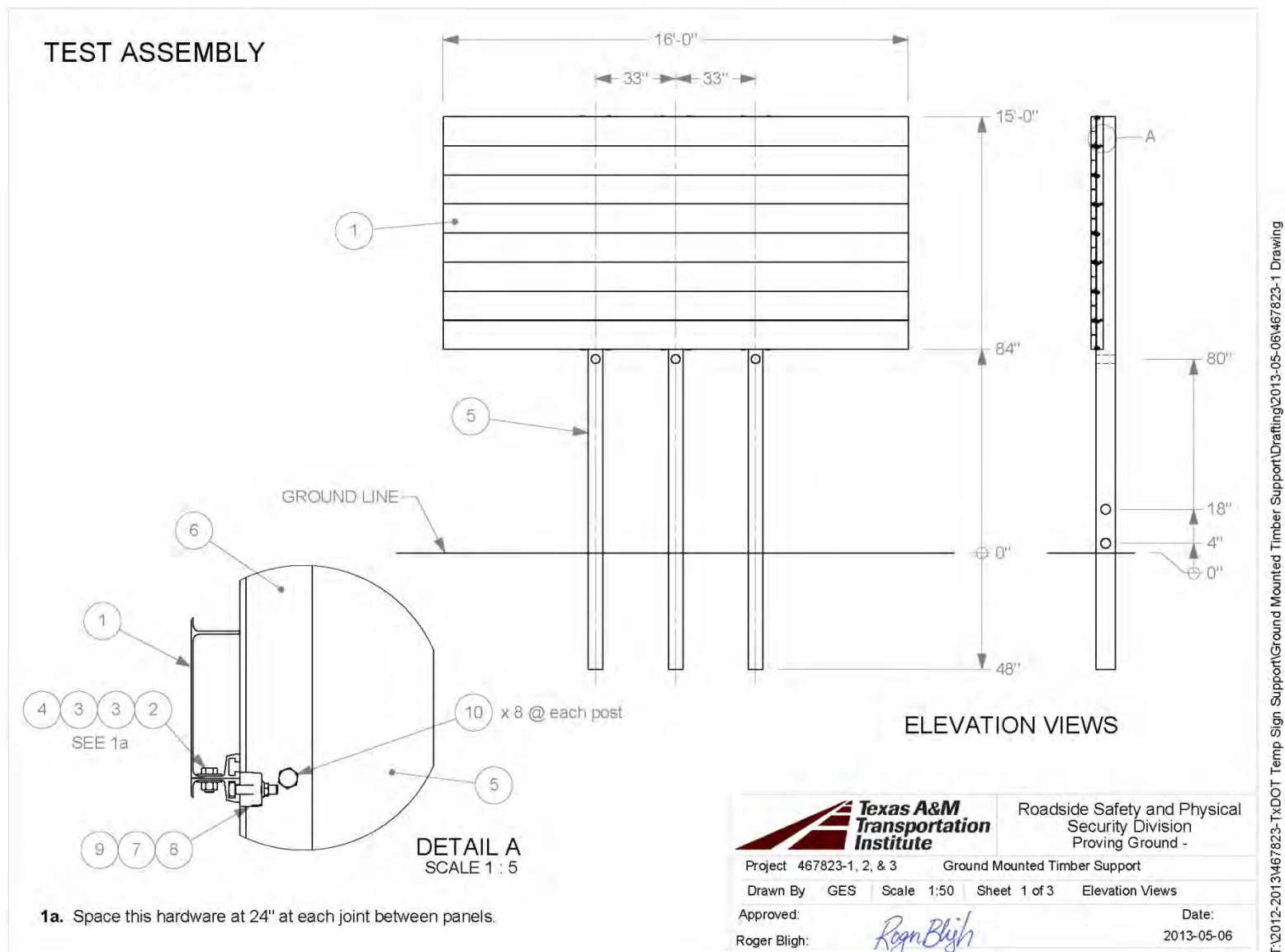
Figure 2.3. Recommended Design for Extruded Aluminum Sign Attached to Direct Embedded Wood Supports.
