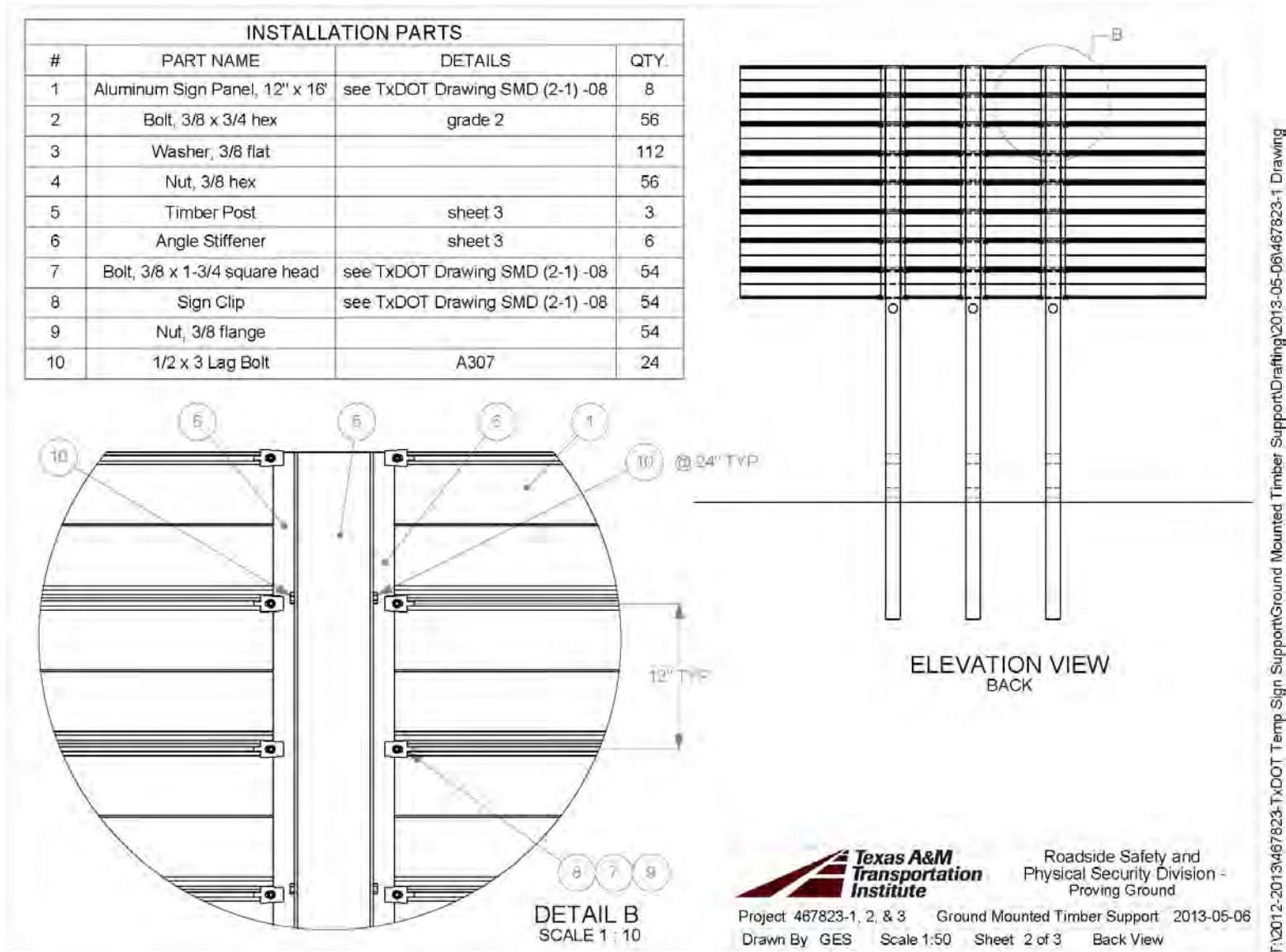
Figure 2.3. Recommended Design for Extruded Aluminum Sign Attached to Direct Embedded Wood Supports (continued).
