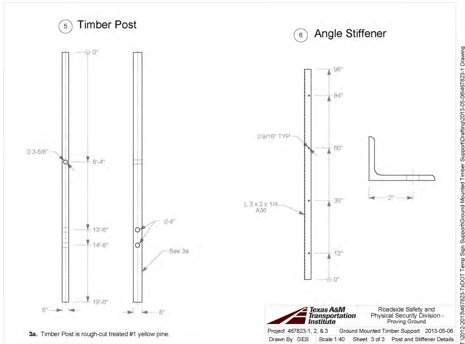
Figure 2.3. Recommended Design for Temporary Large Guide Sign with Direct Embedded Wood Supports (continued).
