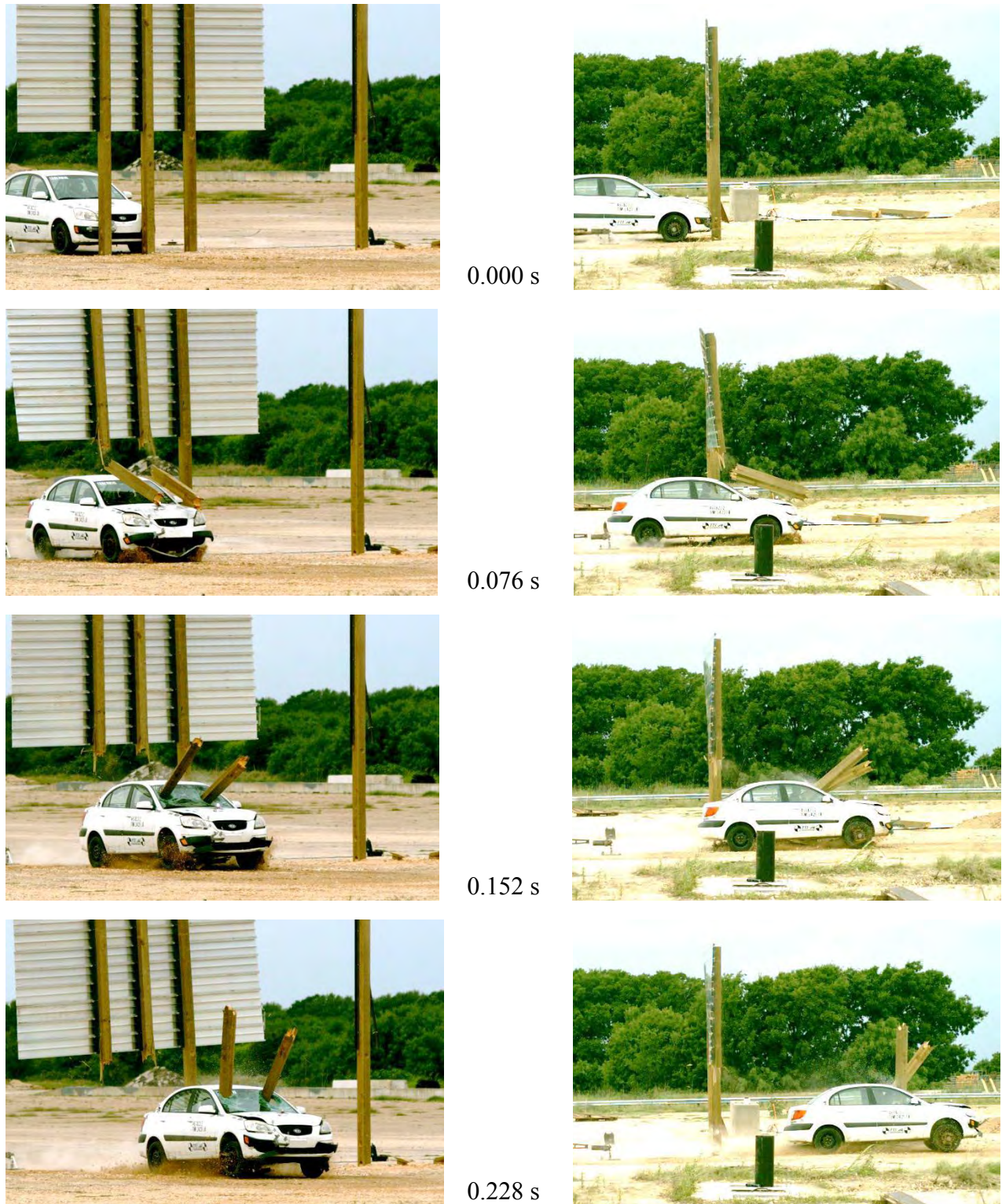
Figure C1. Sequential Photographs for Test No. 467823-2(Oblique and Perpendicular Views).
