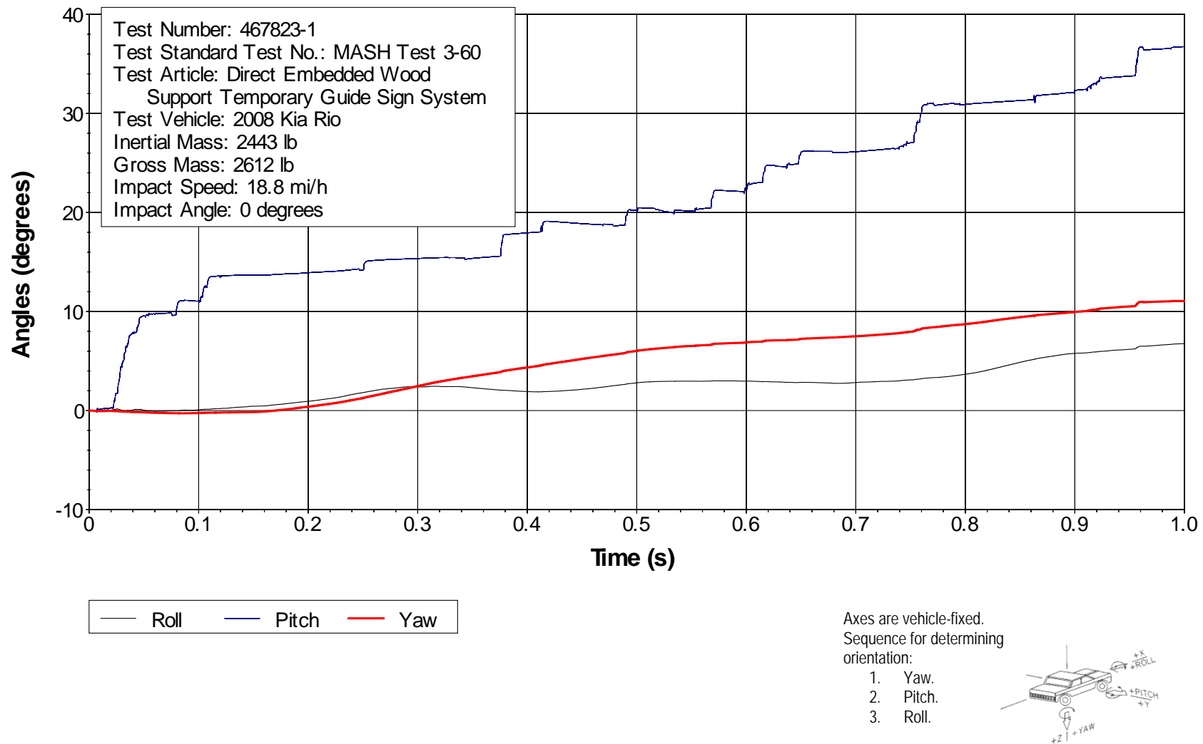
Figure B2. Vehicle Angular Displacements for Test No. 467823-1.
