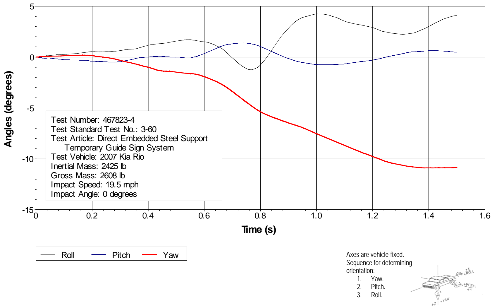
Figure H2. Vehicle Angular Displacements for Test No. 467823-4.
