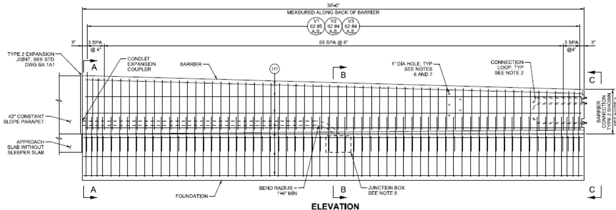
30 ft CIP Concrete Barrier with independent foundation design.
