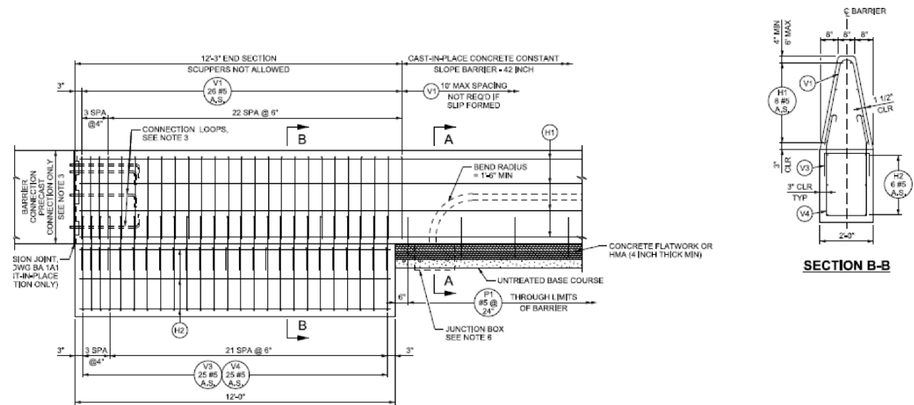
Figure 2: CIP Concrete Barrier placed on asphalt roadway or 4inch thick barrier pad.
