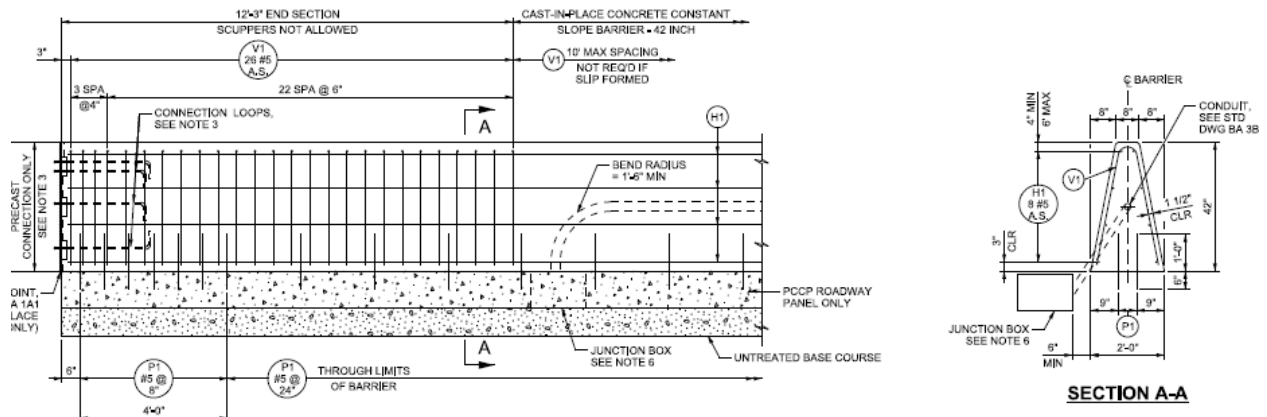
Figure 2: CIP Concrete Barrier placed on asphalt roadway or 4inch thick barrier pad.
